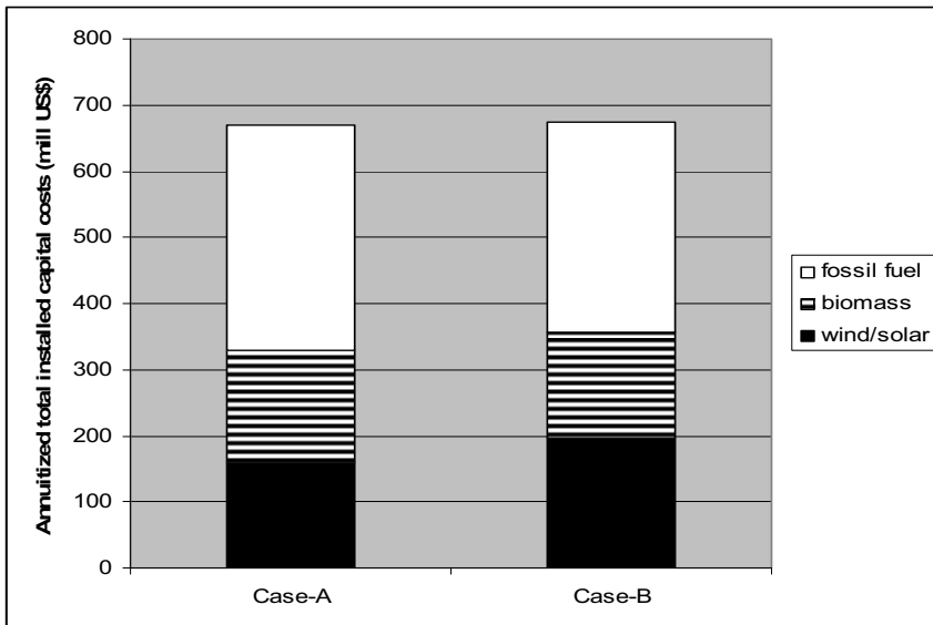
Fig. 6. Cost of the cogeneration system.
