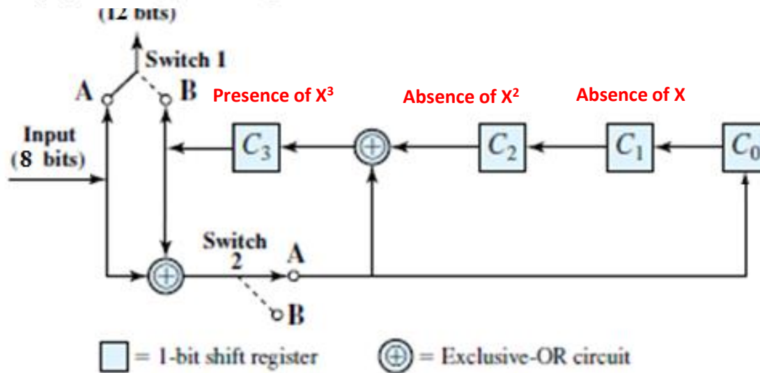
Shift-register implementation
