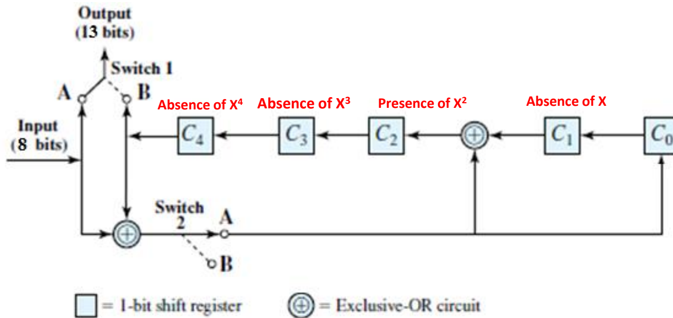
Shift-register implementation
