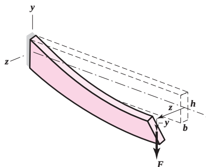
Figure 4-24 Torsional buckling of a thin-walled beam in bending.
