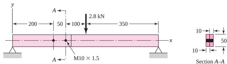
Problem 8–44 Dimensions in millimeters.
