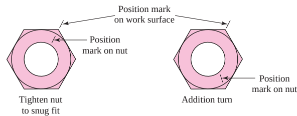
Problem 8-17 Turn-of-nut method
