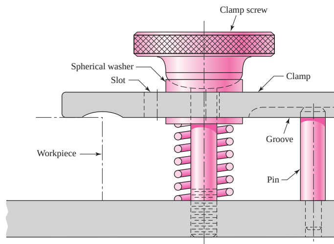
Problem 10-20 Clamping fixture.
