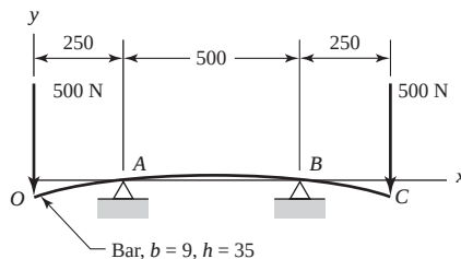
Problem 4-15 Dimensions in millimeters.
