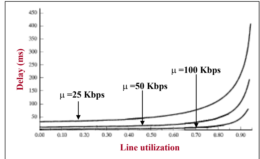
Mean delay versus utilization
