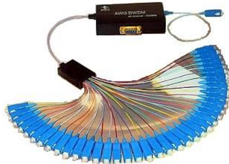
40 channels DWDM
