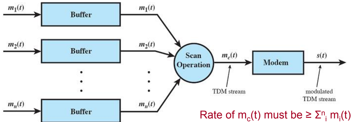
(a) Transmitter
