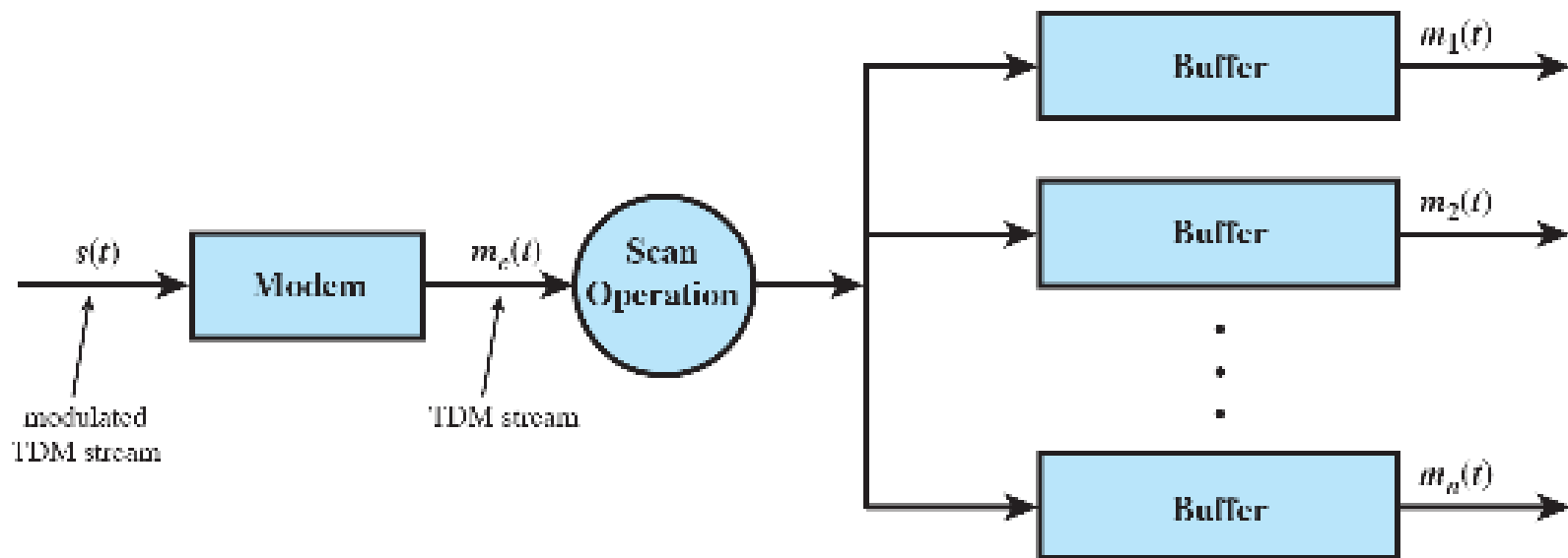
(c) Receiver
