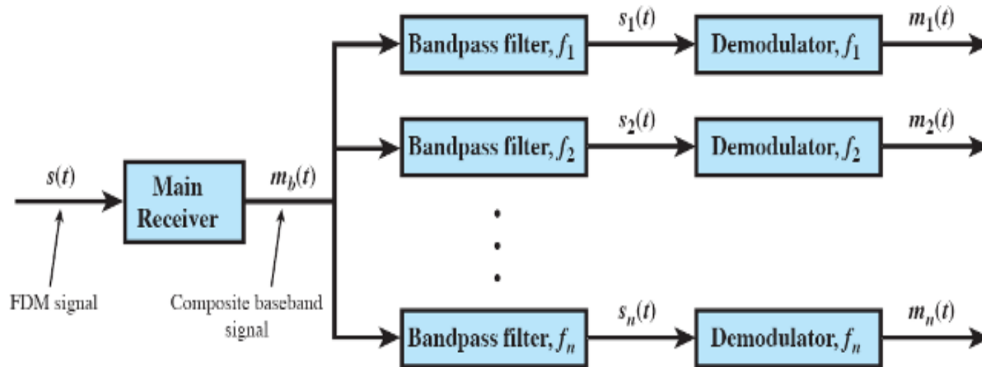
(c) Receiver
