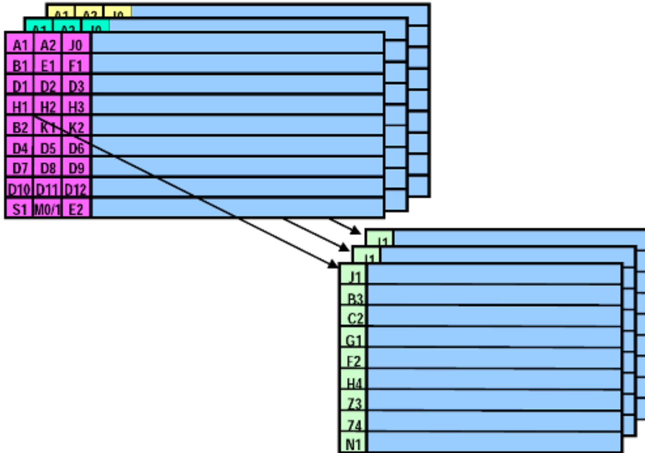
Three individual STS-1 payloads carried in an STS-3 signal
