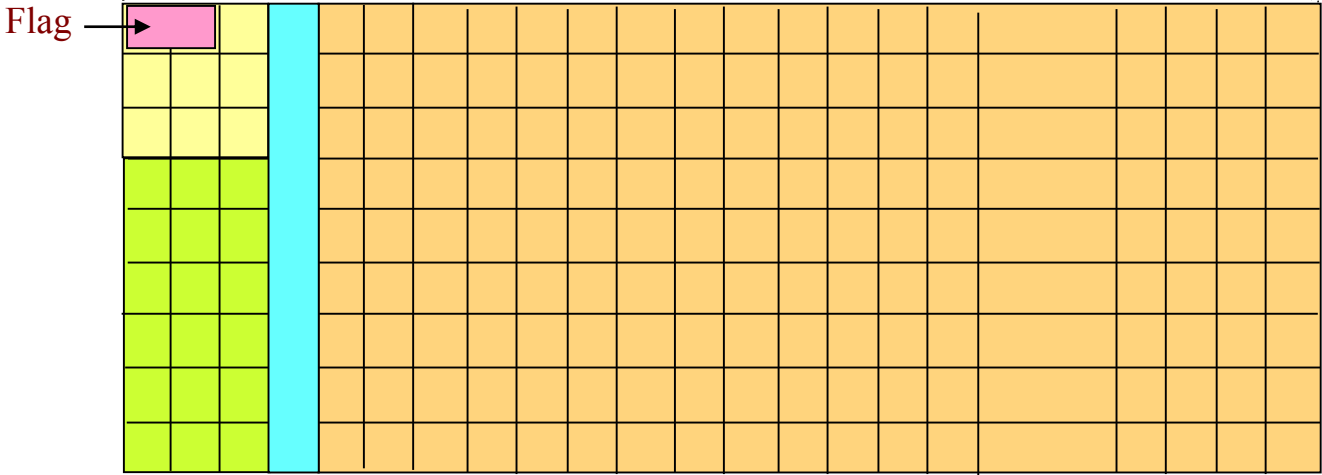
STS-1 Envelope
