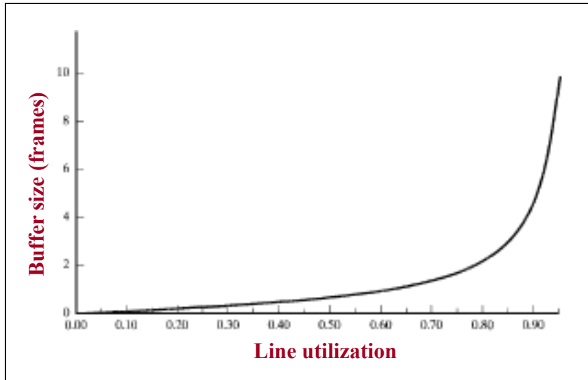
Mean buffer size versus utilization
