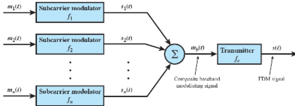
(a) Transmitter
