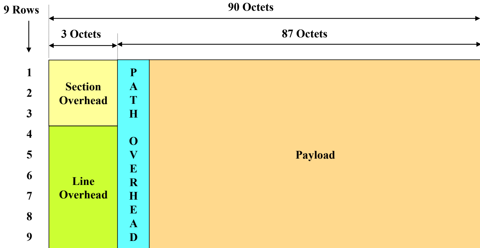
STS-1 Envelope
