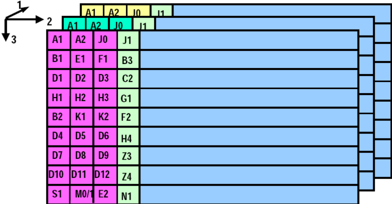
Interleaving of three SONET STS-1 frames into an STS-3 frame
