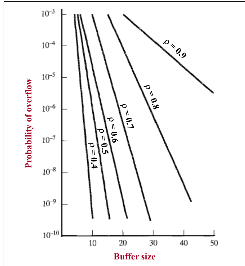
Probability of overflow as a function of buffer size
