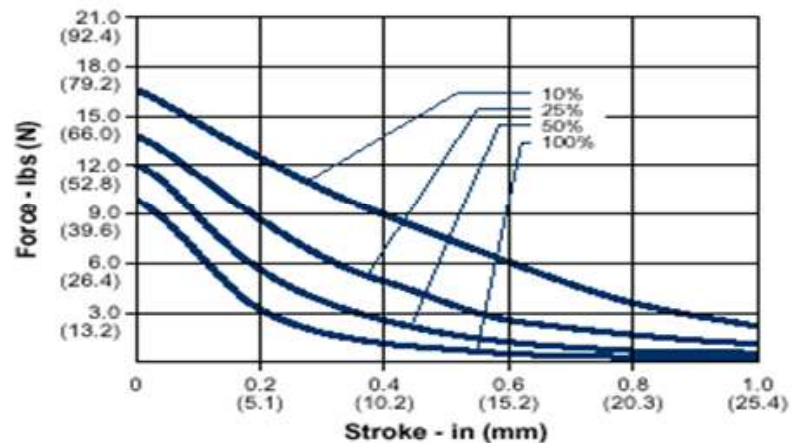
Fig. 5.11 Performance curve for a selected solenoid. [Ledex and Dormeyer Product www.ledex.com ]
