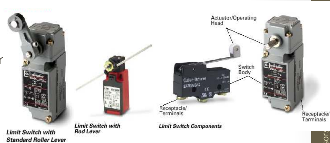
Fig 5.1 Examples of contact switches used as industrial limits switches.
