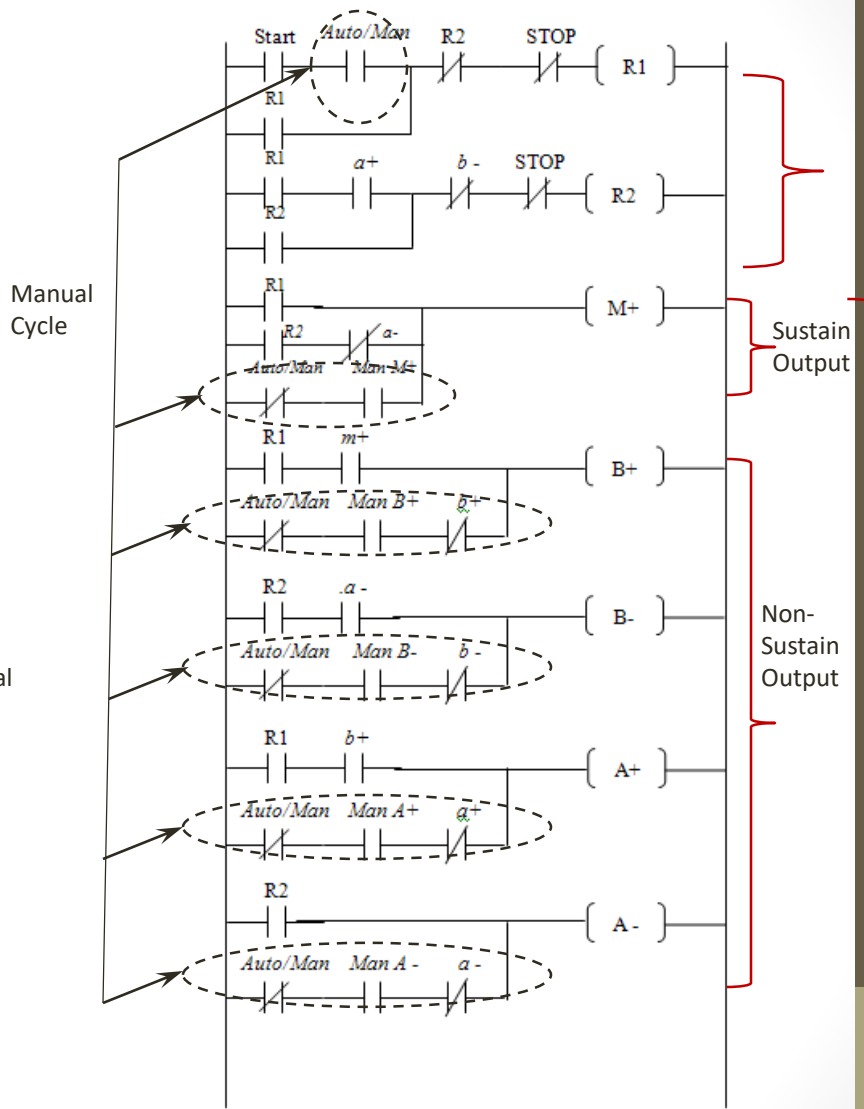
Fig. 9.3 Developed RLL for drilling process automation.
