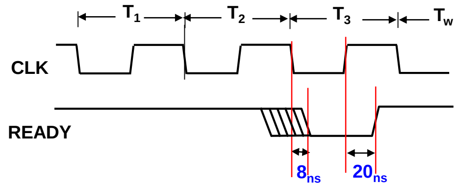
8088-2 READY Input Timing Requirements
